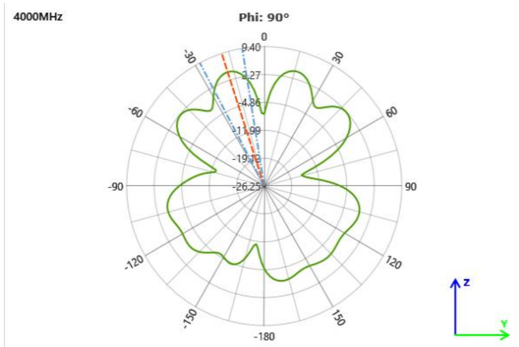
o F=4000MHz Vertical Pattern
