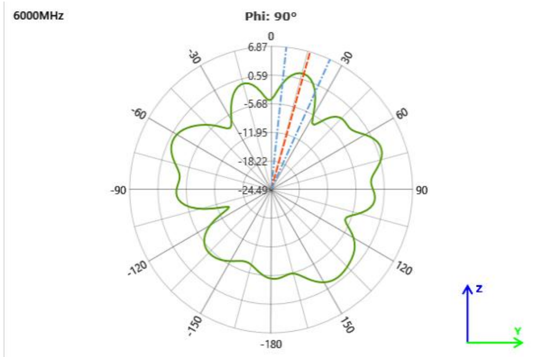
o F=6000MHz Vertical Pattern
