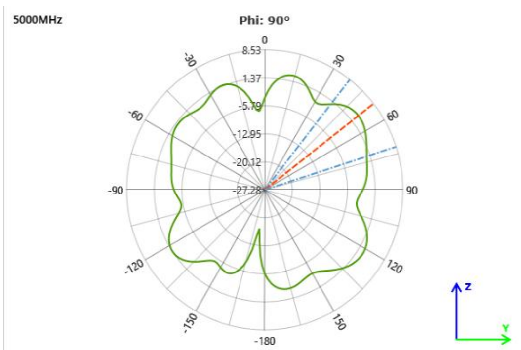
o F=5000MHz Vertical Pattern
